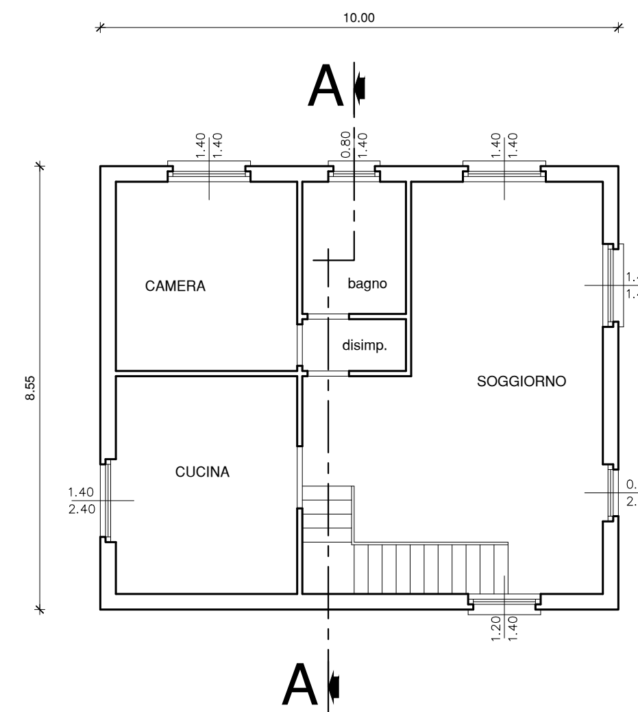
Piano terreno
